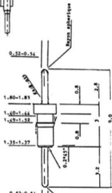
—9.0m/m— MALE PIN
